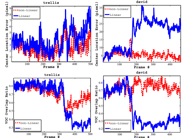
Figure 7: Quantitative comparison of the proposed tracker with/without non-linear extension on two videos. The left two subfigures are associated with the tracking performance in CLE and VOR on the trellis video, respectively; the right two subfigures correspond to the tracking performance in CLE and VOR on the david video, respectively.
