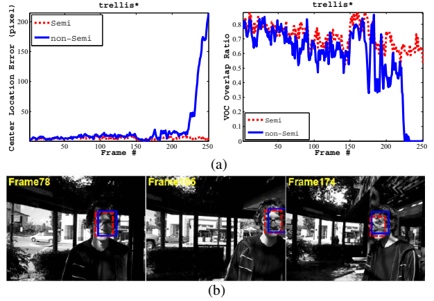
Figure 6: Comparison of the proposed tracker with/without semi-supervised learning on the trellis* video. (a) shows tracking performance in CLE and VOR; (b) shows some screenshots, red dashed line indicates scenario with semi-supervised learning, blue line indicates without.
