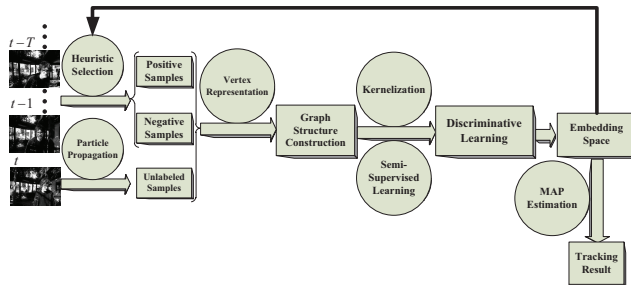
Figure 2: The architecture of the tracking framework.
