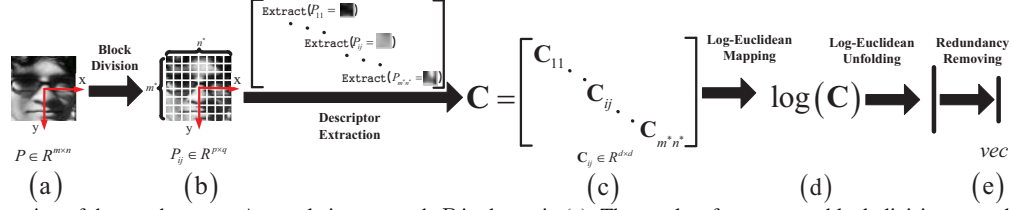
Figure 3: Representation of the graph vertex. A sample image patch P is shown in (a). The results of appearance block division are exhibited in (b), where m^* is denoted as \lceil m/p \rceil , n^* is denoted as \lceil n/q \rceil , and \lceil \cdot \rceil is denoted as the rounding operator. The block-division based covariance matrix descriptor \mathbf{C} is shown in (c). The Log-Euclidean mapping and unfolding are displayed in (d) and (e).
