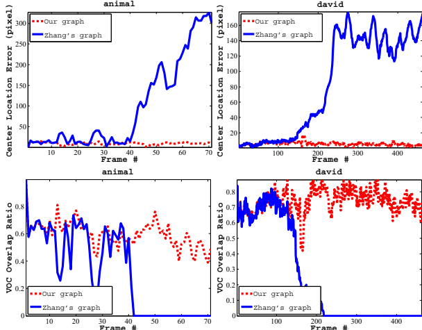
Figure 5: Quantitative comparison of the proposed tracker with our new graph and Zhang’s graph [26] on two videos. The left two subfigures are associated with the tracking performance in CLE and VOR on the animal video, respectively; the right two subfigures correspond to the tracking performance in CLE and VOR on the david video, respectively.
