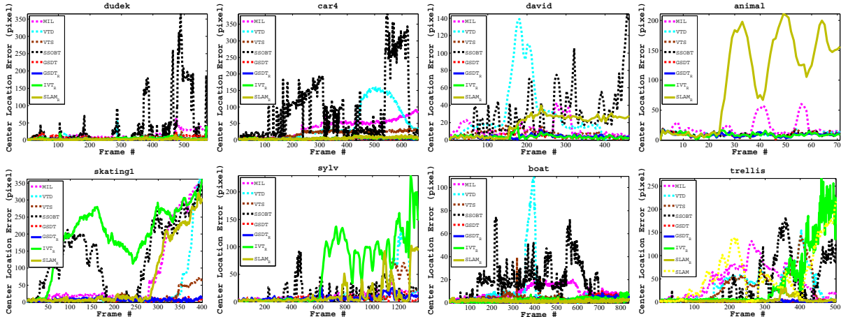
Figure 8: Quantitative comparison of different trackers in terms of CLE on eight videos.
