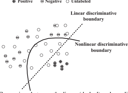
Figure 4: Comparison between the linear (dashed) and non-linear (solid) discriminative boundary.
